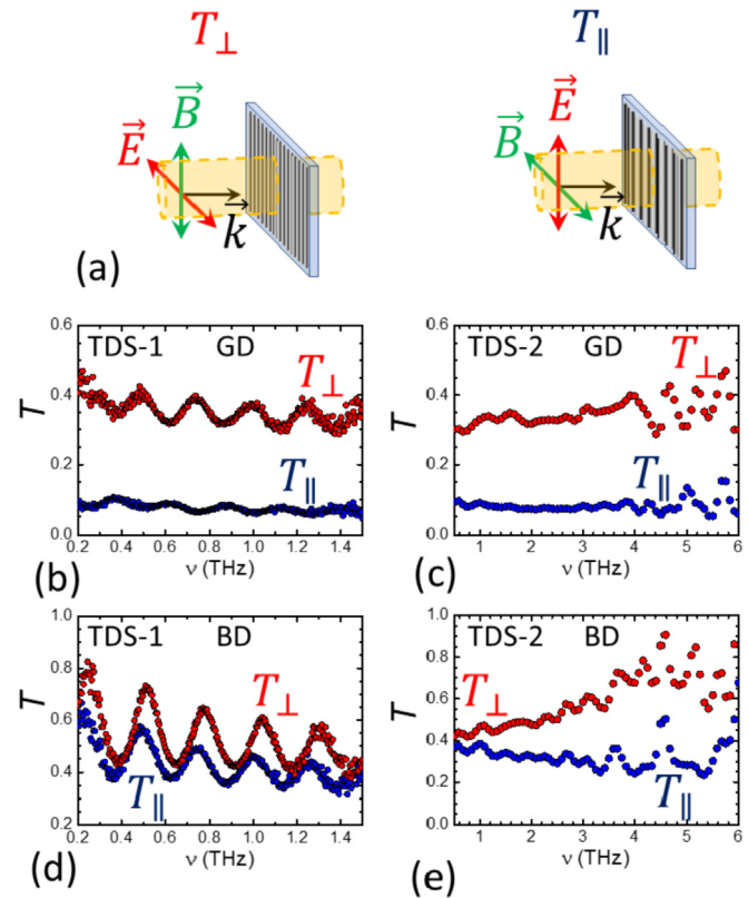
Fig. 3. Panel (a): sketch of the THz wave for THz electric field polarization orthogonal ( T_{\perp} , red symbols) parallel ( T_{\parallel} , blue symbols) to the LIPSS. Panel (b–e): transmittance of graphitized (b–c) and black (d–e) diamond as taken using TDS-1 (left) and TDS-2 (right) setups. (A colour version of this figure can be viewed online.)
