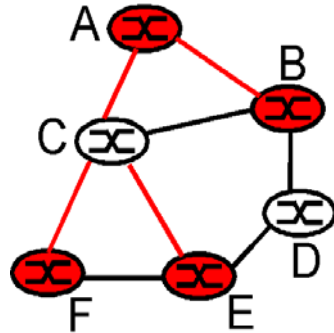
Group-shared Tree
