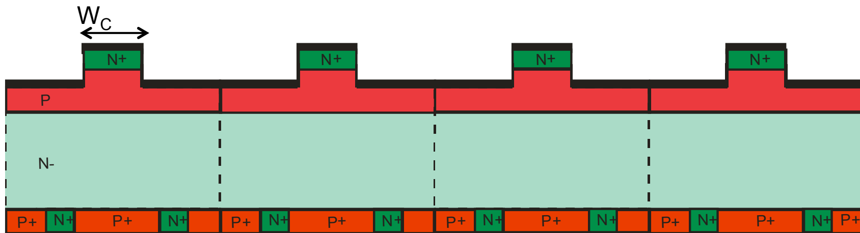
GTO cross-section
