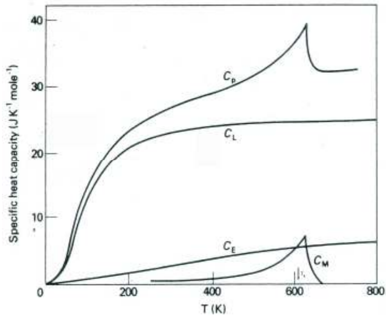
Heat capacity of Ni
