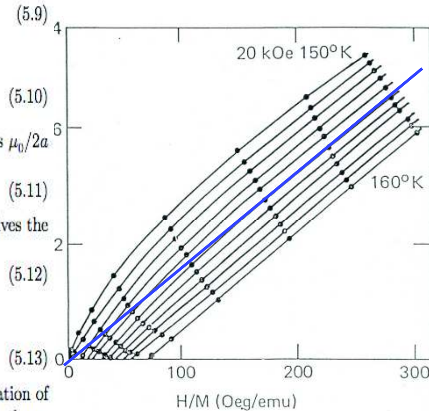
Arrott plots
