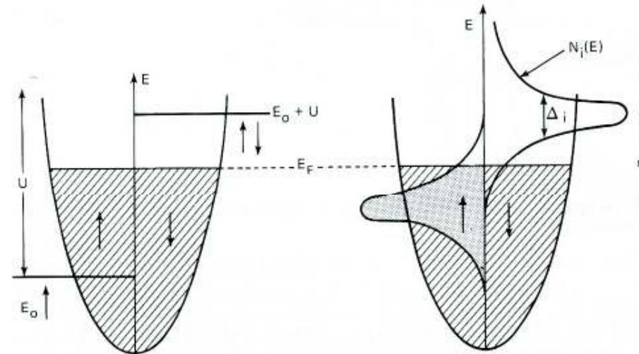
No hybridization
