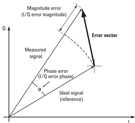
Figure 11. Error vector and related parameters
