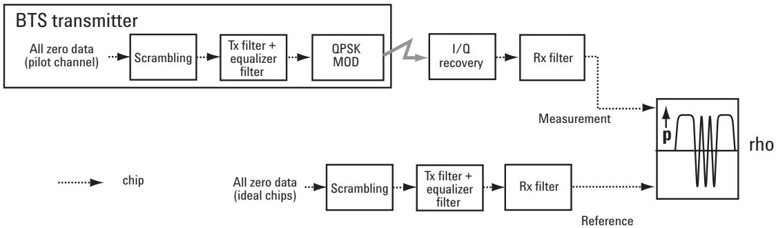
Figure 15. Traditional process to calculate rho for a cdmaOne or cdma2000 SR1 forward link pilot-only signal
