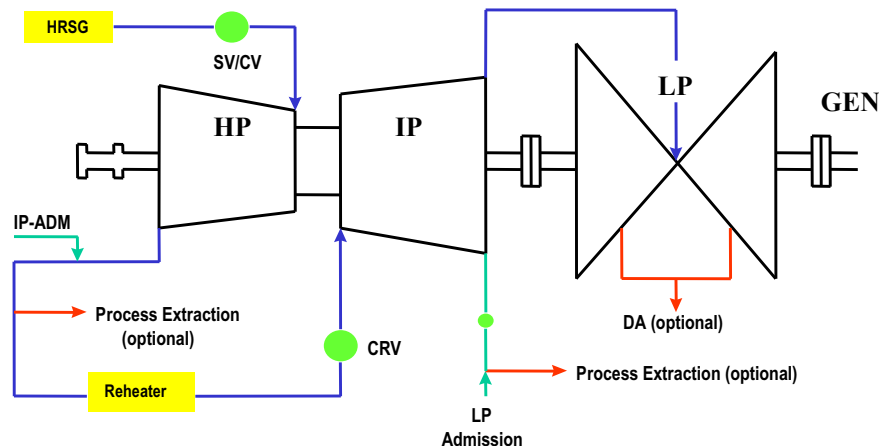
Figure 12. Schematic showing structured D-11 layout with possible extractions
