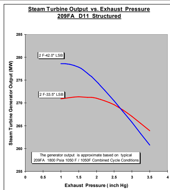
Figure 11b. Output vs. exhaust pressure – 50 Hz
