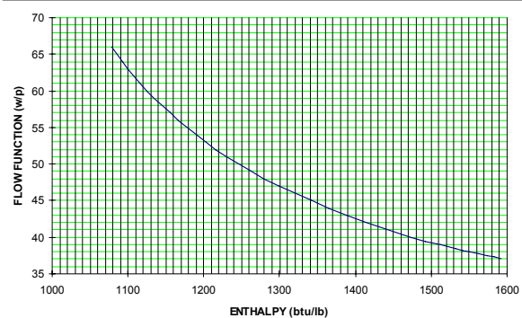
Figure 10. Flow function vs. enthalpy
