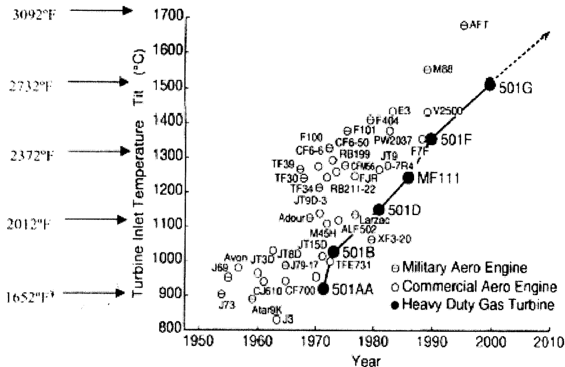
Figure 1. Aero and industrial GT Industry Trend
